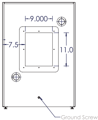
24" Wide (1 DOOR)
