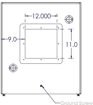
30" Wide (2 DOOR)
